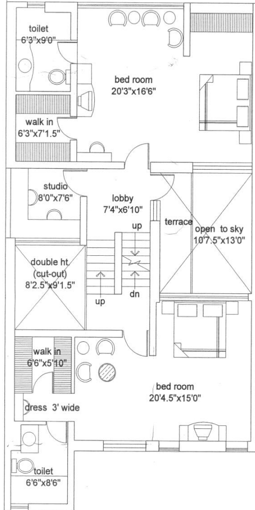
FIRST FLOOR PLAN [OPTION -2]
