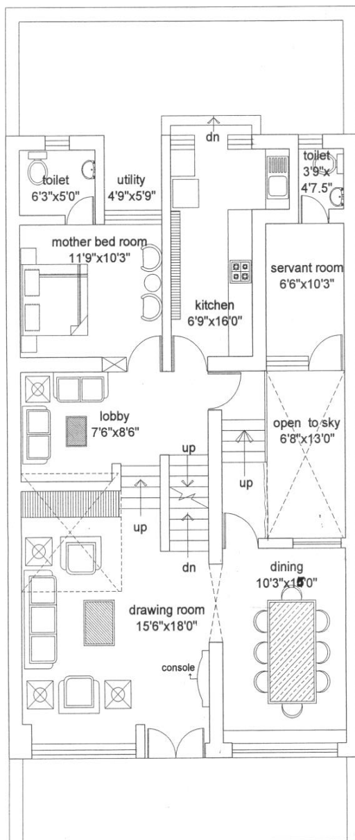
GROUND FLOOR PLAN [OPTION -2]
